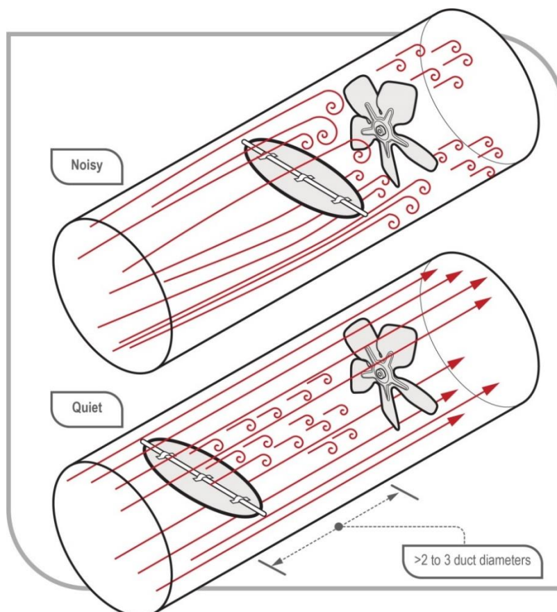
Figure 5 High pressure and low air pressure combine to cause noise
