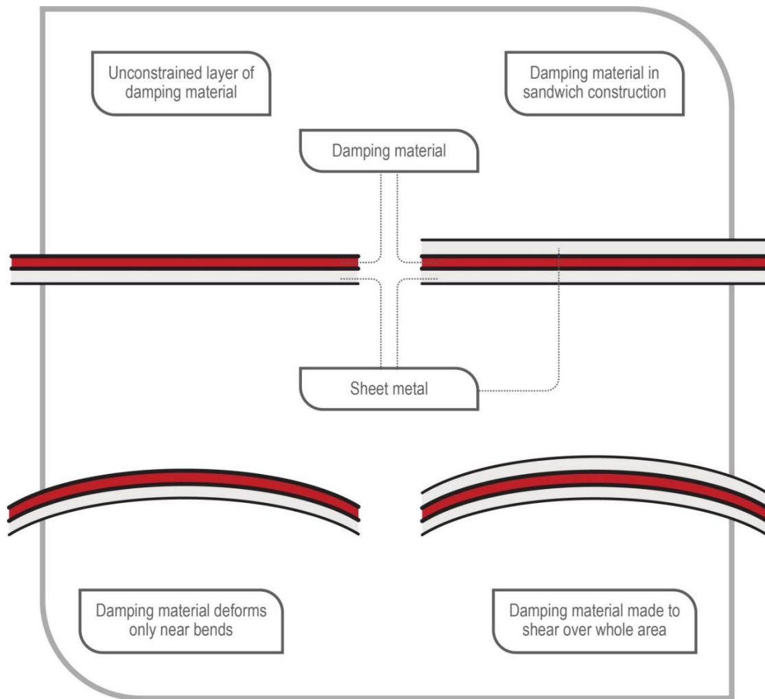
Figure 4 Damping
