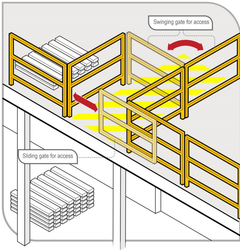
Figure 3 Mezzanine floor barrier
