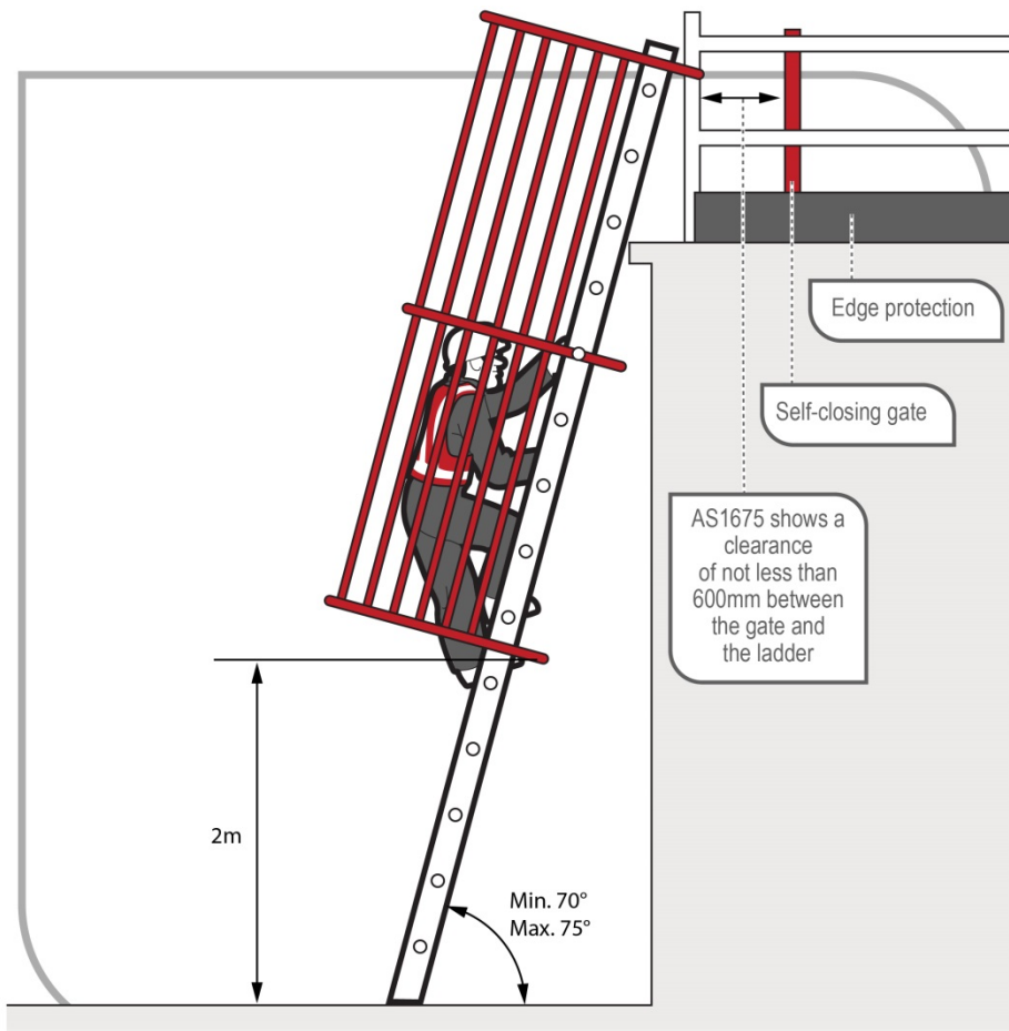
Figure 32 Fixed ladder with ladder cage
