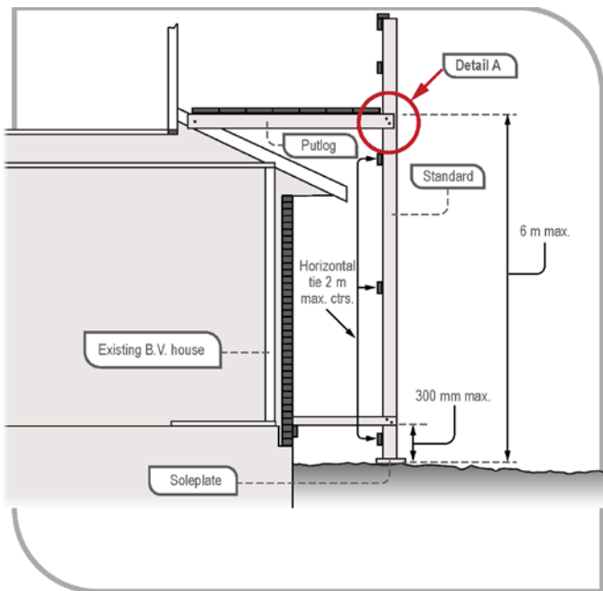
Figure 30 Timber scaffold (single pole – high first lift)
