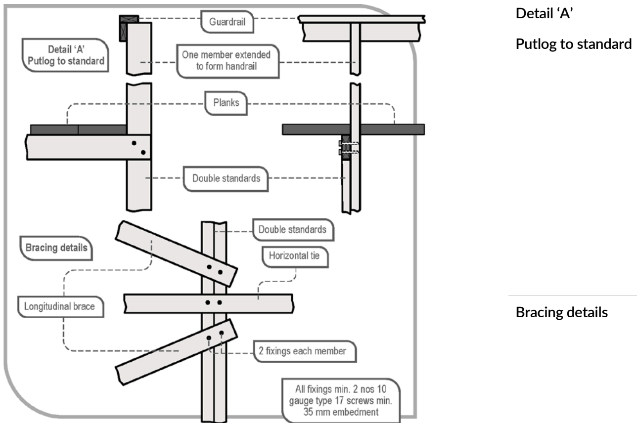
Figure 31 Timber scaffold (single pole - high first lift) details
