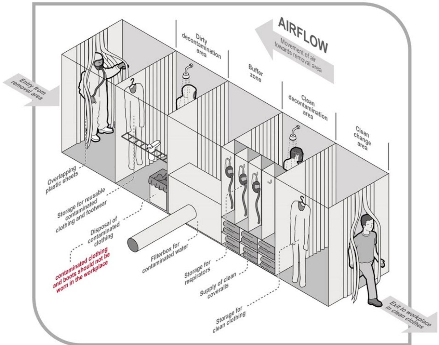
Figure 4 Decontamination unit
