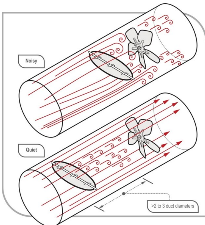
Figure 6 Damper further from fan is quieter
