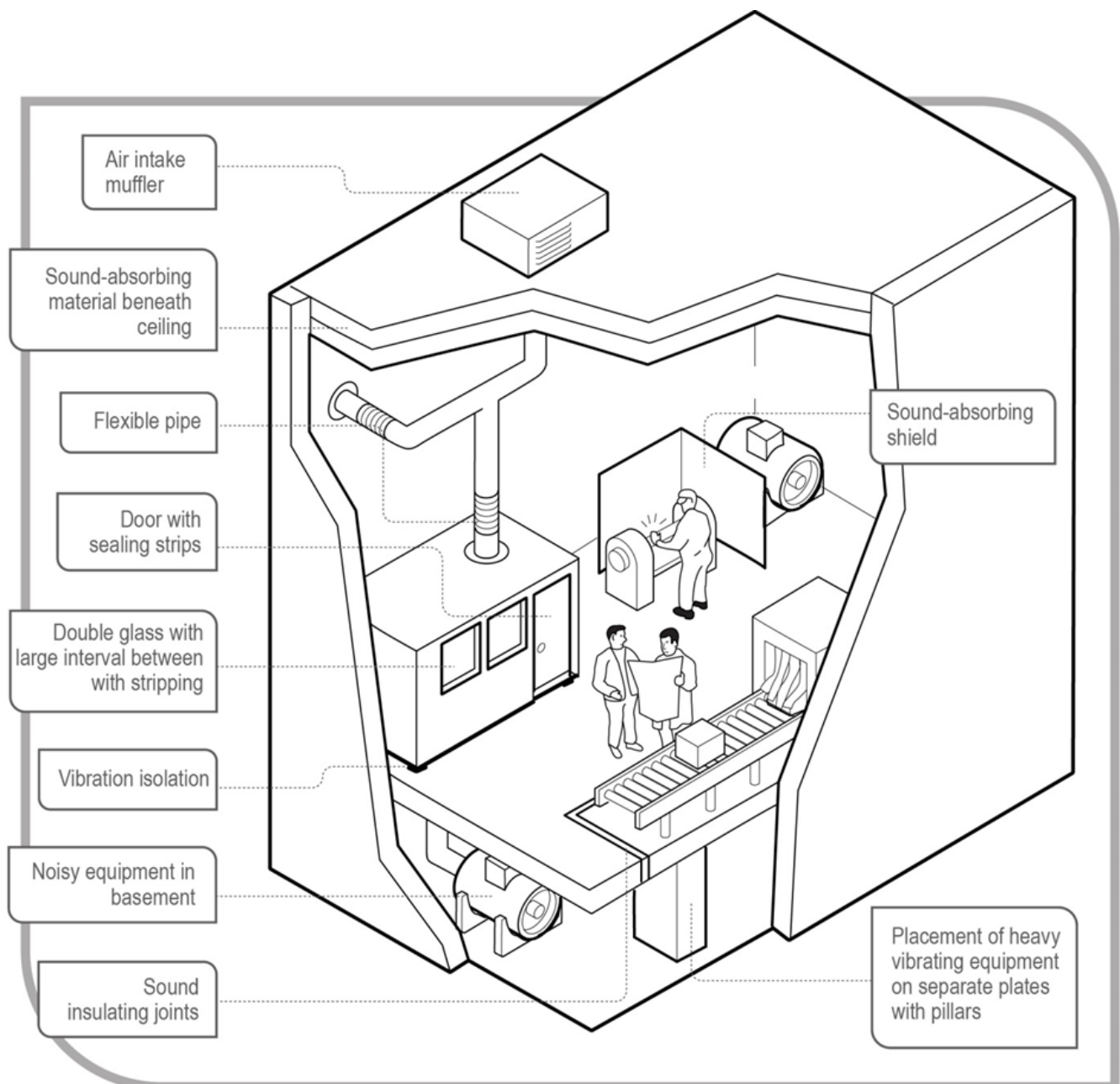
Figure 3 Examples of noise control measures in an industrial building
