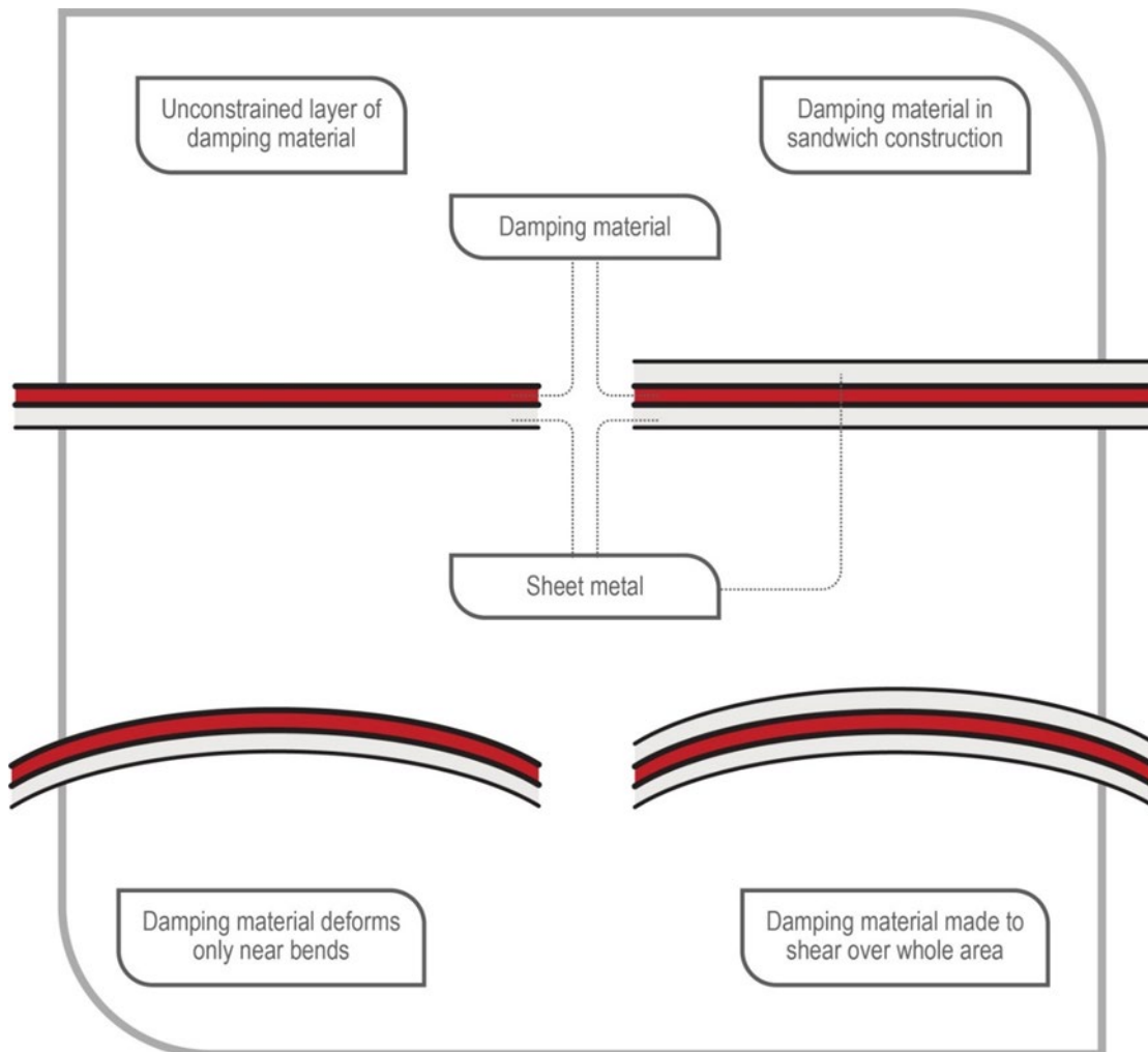
Figure 4 Damping
