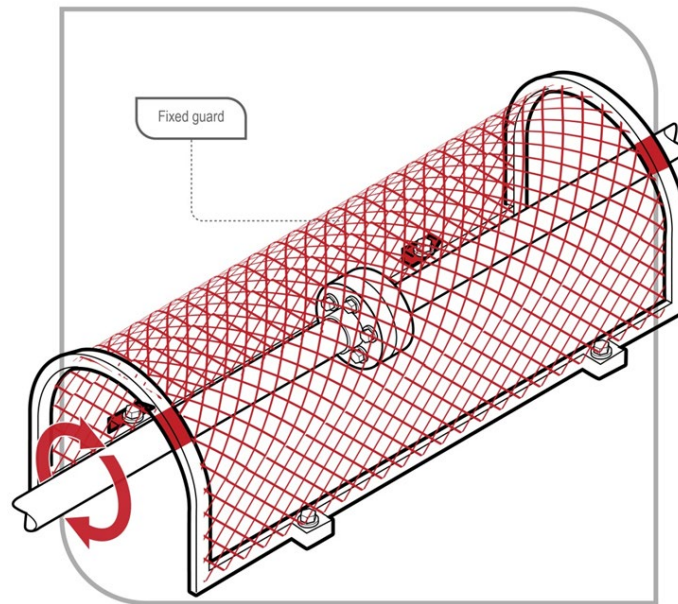
Figure 3 Fixed guard on rotating shaft or coupling
