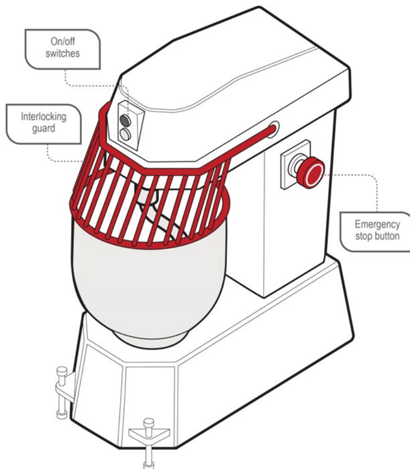
Figure 2 Food mixer with interlocking guard
